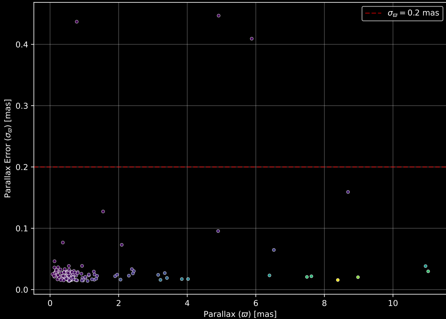
APOGEE DR17 Field: [M4] Parallax Quality (n= 185)
