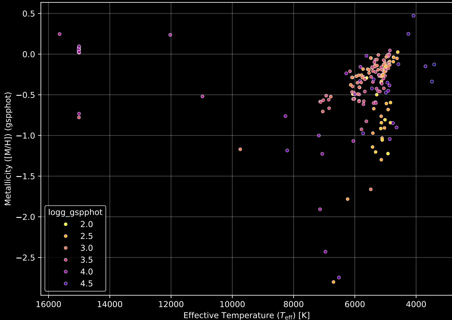
APOGEE DR17 Field: [M4] Stellar Population Parameters (n= 185)
