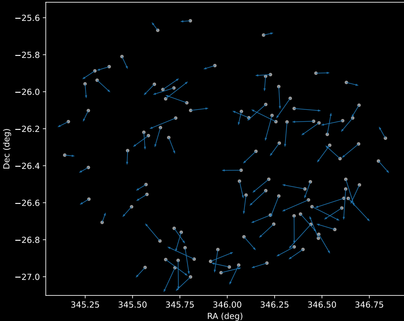
APOGEE DR17 Cluster 0 Proper Motion Vectors (n=99)
