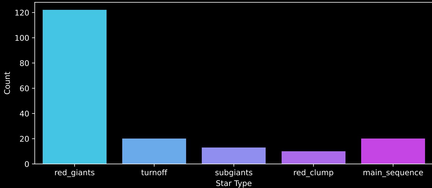
APOGEE DR17 Field: [M4] Count plot of Star Type
