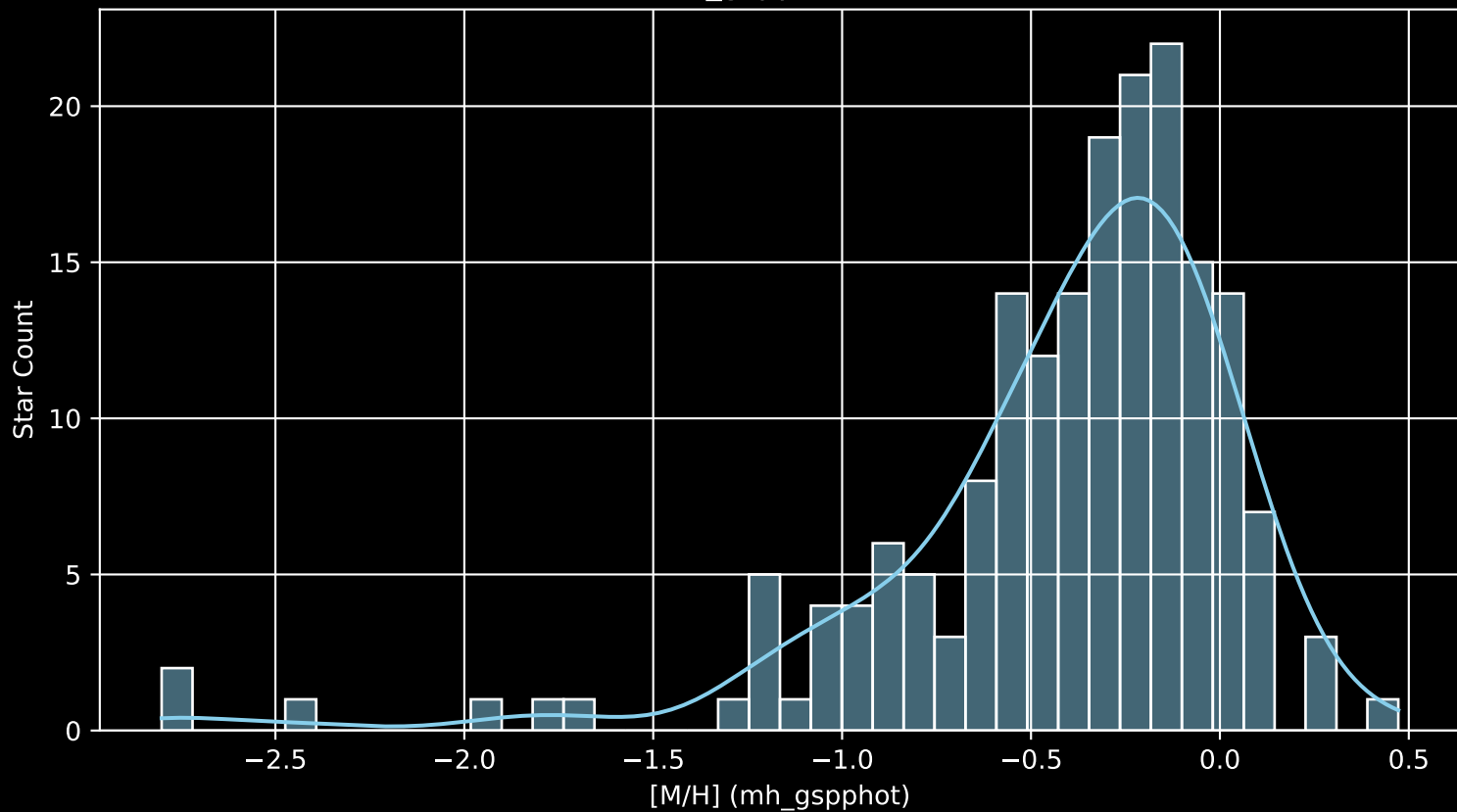
APOGEE DR17 Field: [M4 [M/H] (mh_gspphot) (n= 185)
