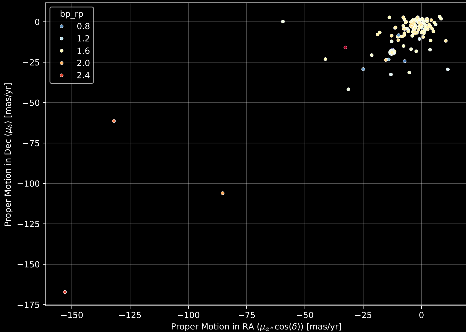
APOGEE DR17 Field: [M4] Proper Motion Diagram (n= 185)
